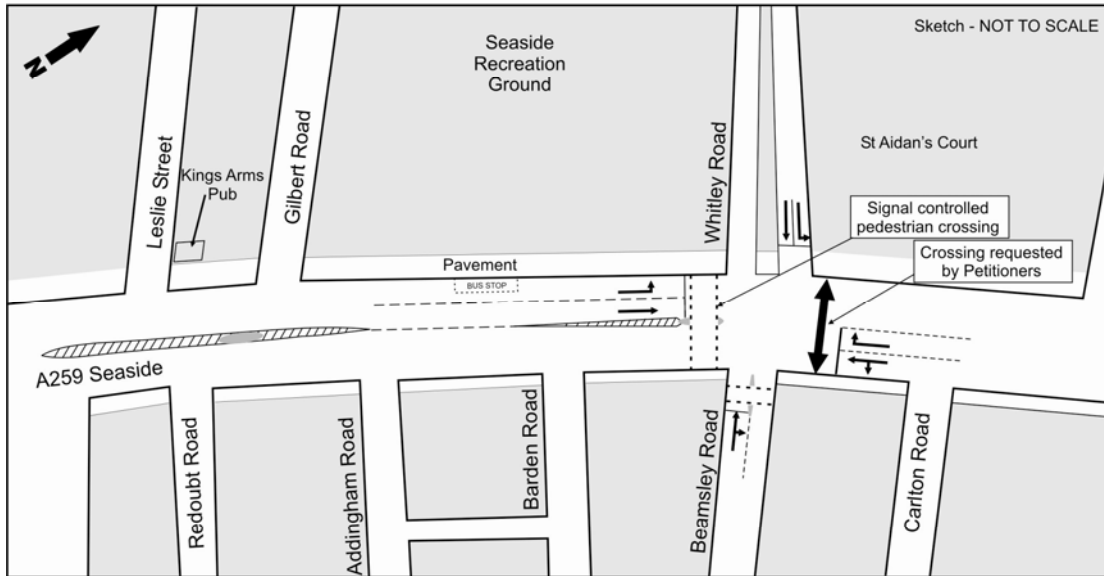
Figure 1. Existing junction layout
