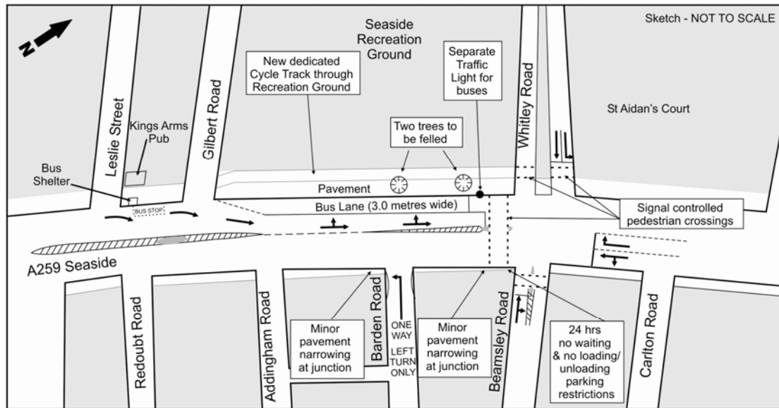
Figure 2. Seaside Quality Bus Corridor Phase 1 Scheme Proposed bus lane and dedicated cycle track through Recreation Ground
